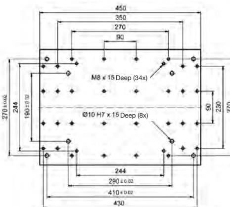
Hole pattern table length 450:
