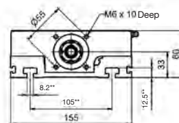
Hole pattern table length 220 mm:
