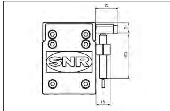
Mounting option 4
