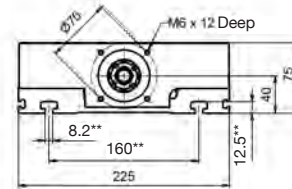
Hole pattern for table length 320:
