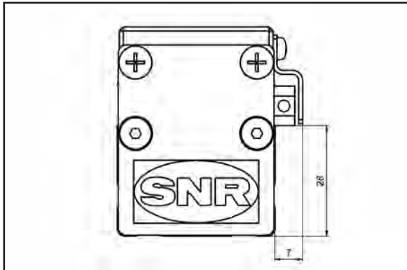
Mounting option 3
