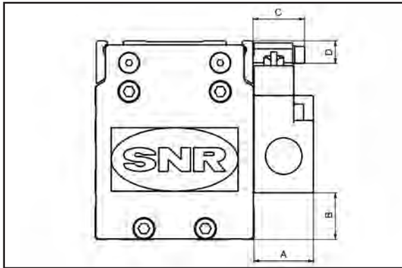
Mounting option 1
