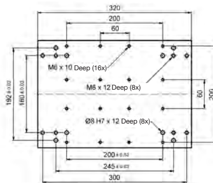
Hole pattern for table length 320:
