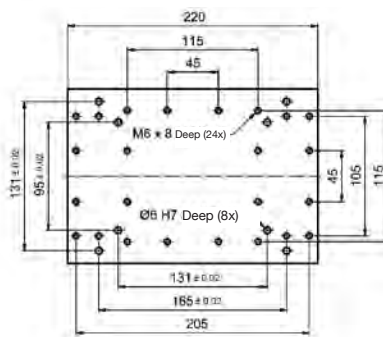
Hole pattern table length 220 mm:
