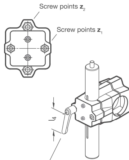
Adjustable hand lever HSK
