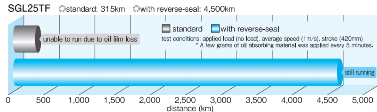
Figure A-35 Grease Dry-up Test Data
