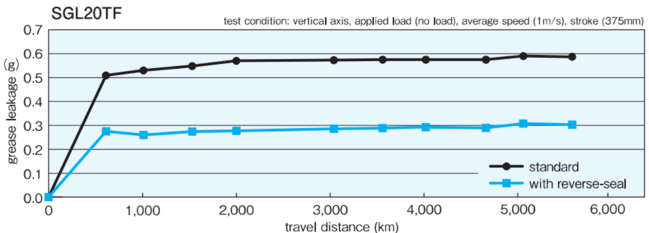
Figure A-34 Grease-leak Test Data
