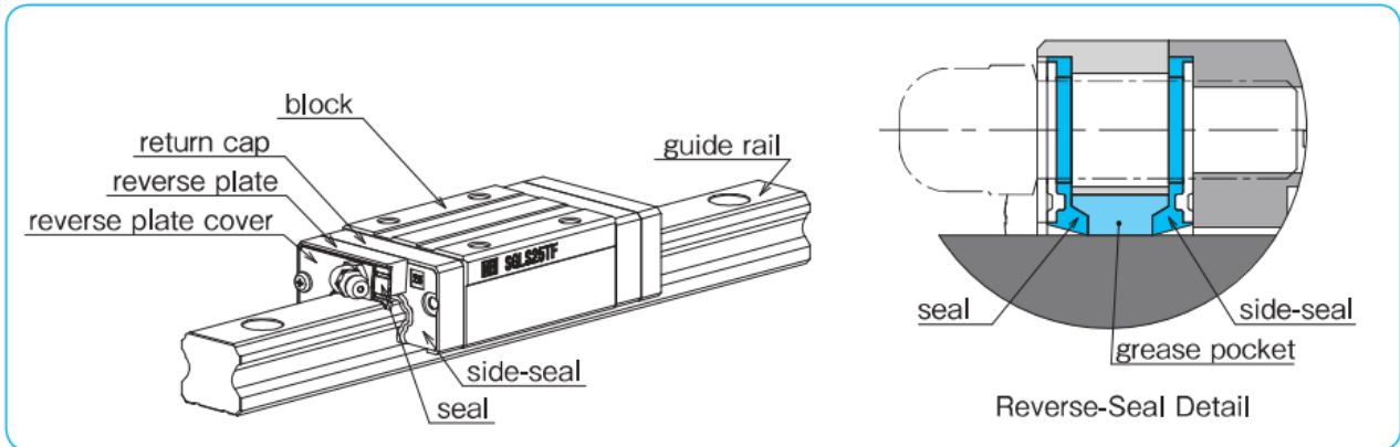
Figure A-33 Reverse-Seal
