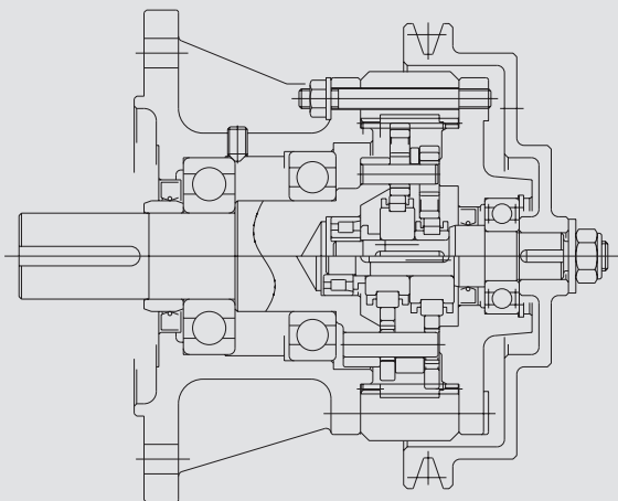
Circulute Pulley, Flange Mount
