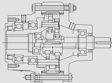
Shaft Input w/Hollow Shaft Output
