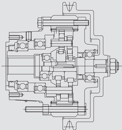
Circulute Pulley w/Hollow Shaft
